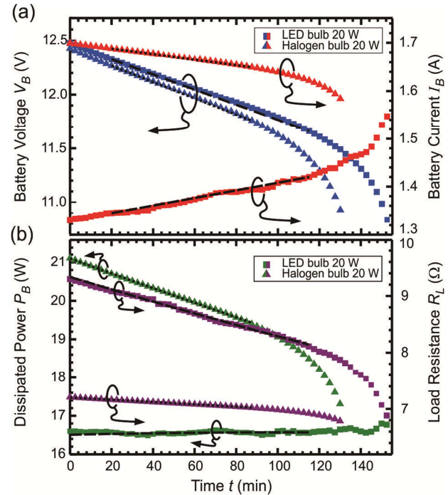
Fig. 4 (a) The battery voltage and battery current and (b) dissipated power and load resistance during discharge of lead-acid battery via discharge controller. A 20-W LED bulb and halogen bulb are used as a load.
