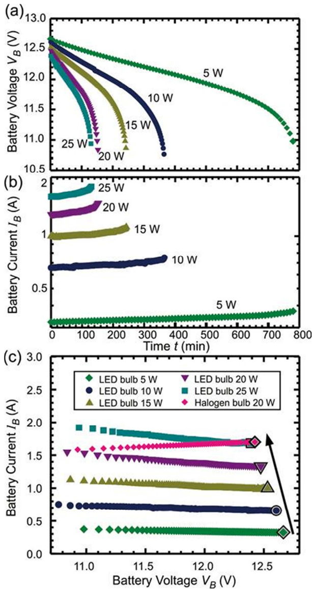
Fig. 3 (a) battery voltage and (b) battery current during discharge of a lead-acid battery at different load size of LED bulbs. (c) I-V characteristics of various types of light bulb.
