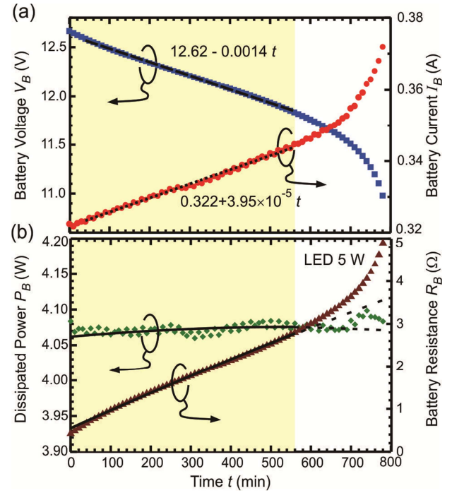
Fig. 2 (a) The battery voltage and battery current and (b) dissipated power and battery resistance during discharge of lead-acid battery via discharge controller. A 5-W LED bulb is used as a load.
