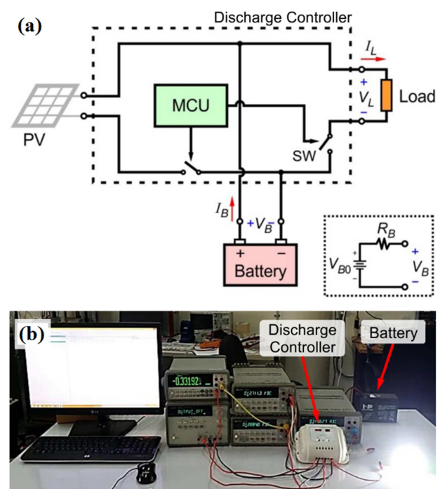
Fig. 1 (a) Block diagram of the investigated system consists of a discharge controller, battery and load. The lower right inset is the equivalent circuit of battery. (b) The photograph of the investigated system.
