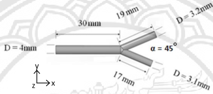
Figure 1 Computational domain and dimensions
