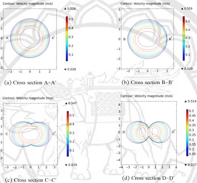
Figure 4 Velocity contours in the main vessel and the bifurcation junction at peak systole ( Re = 750 ).
