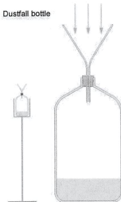
Figure 1: Typical dust fall bottle set-up
